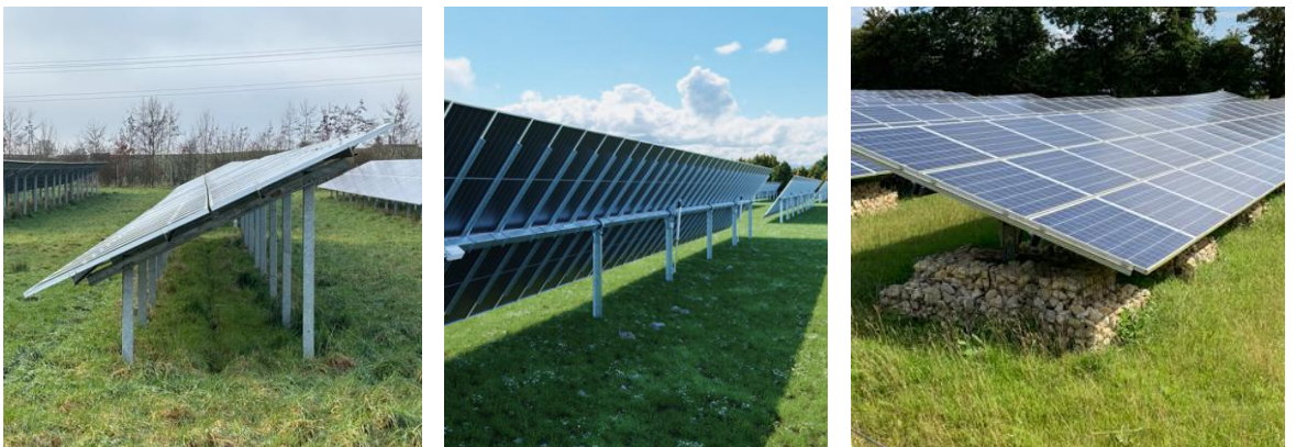
Figure 15.13-14 Examples of Solar PV Generating Station Fixings
