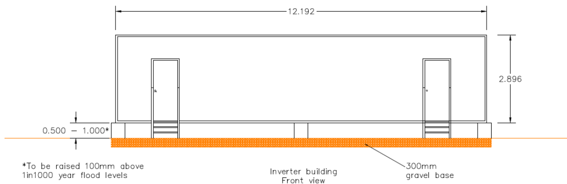
Figure 15.16-17 Typical Inverter Front Elevation
